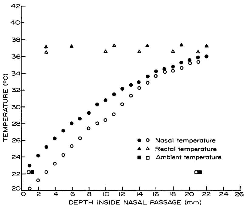
FIGURE 5 Temperature in nasal passage of kangaroo rat as a function of depth inside passage. Open symbols represent 37% relative humidity and closed symbols, 62.5%.
